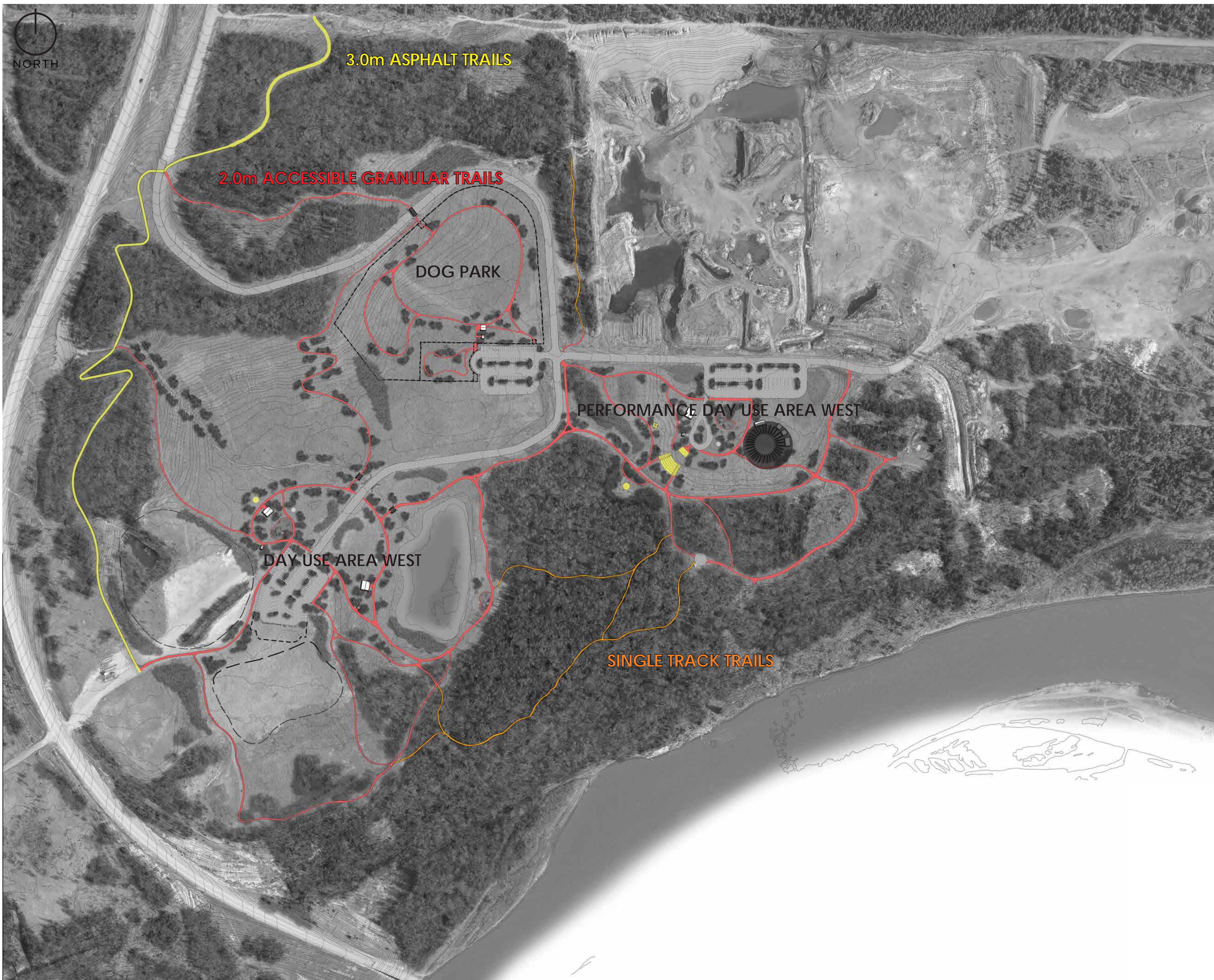
3.0m WIDE ASPHALT TRAIL
